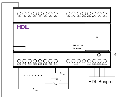
Figure 4. Wiring
