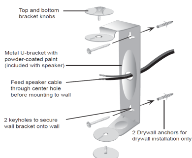
Figure 6. Wall-mount speaker bracket
