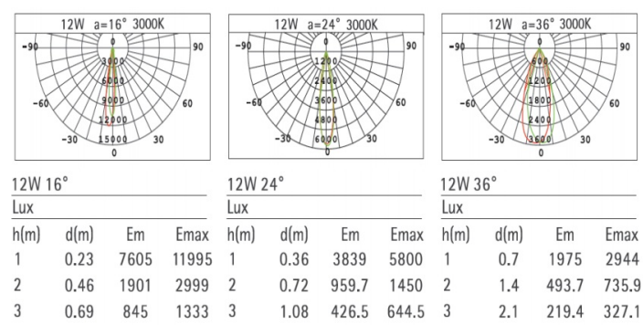
Figure 2- Adjustable Color Temperature - Light Distribution
