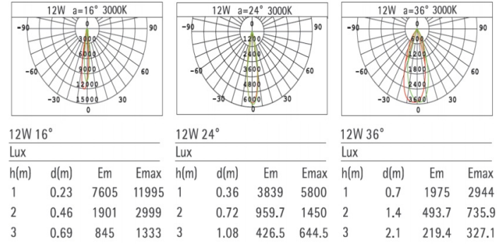
Figure 3- Fixed Color Temperature - Light Distribution
