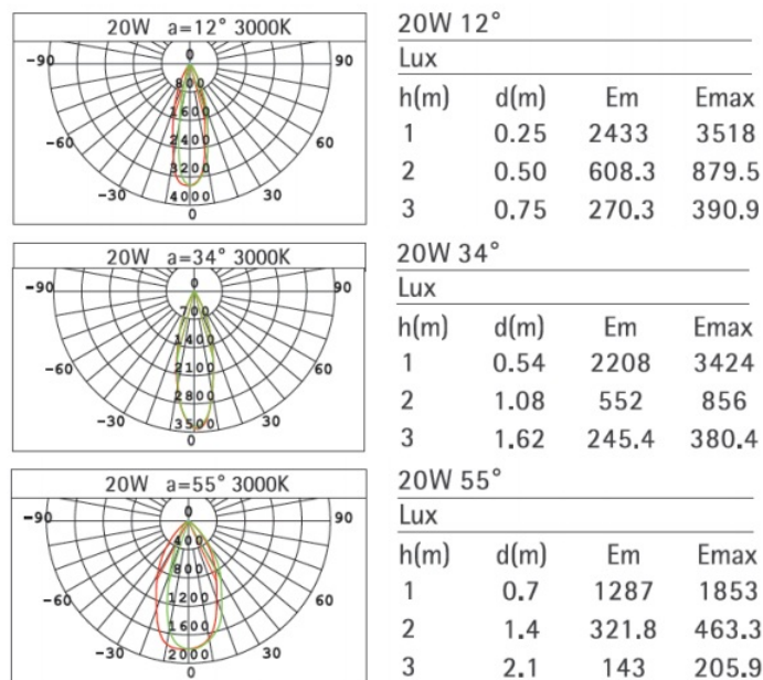
Figure 3- Fixed Color Temperature - Light Distribution
