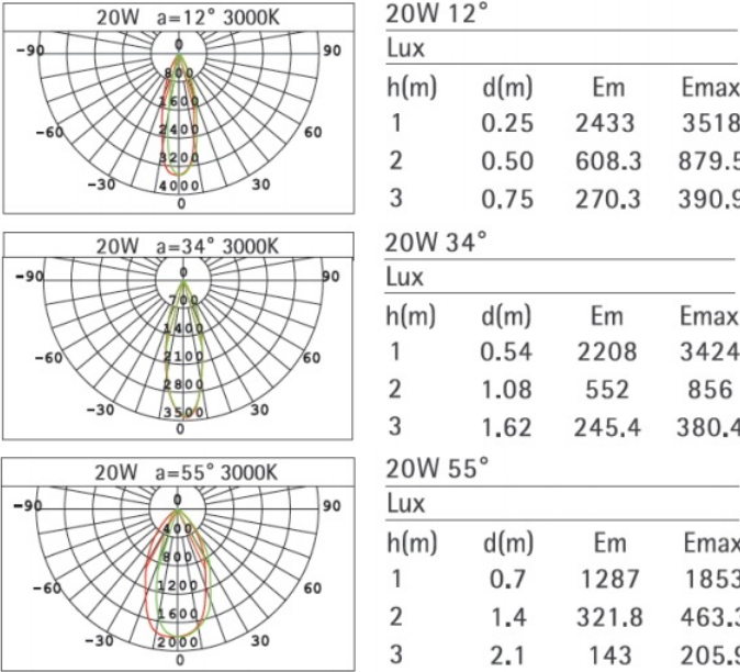
Figure 2- Adjustable Color Temperature - Light Distribution
