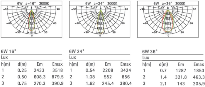
Figure 2- Adjustable Color Temperature - Light Distribution
