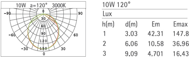
Figure 2- Adjustable Color Temperature - Light Distribution
