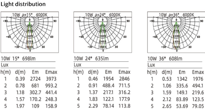
Figure 2- Adjustable CCT Light - Light Distribution
