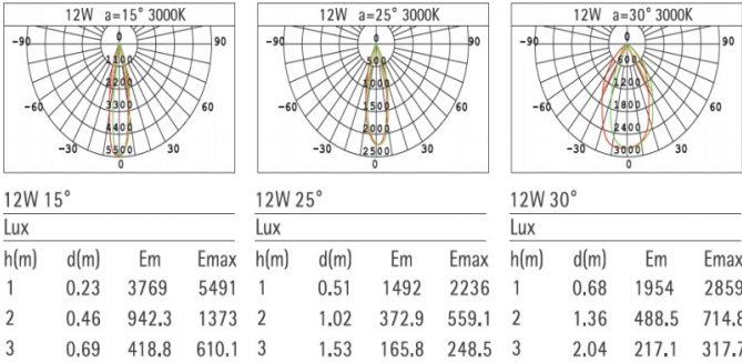
Figure 3- Fixed CCT Light - Light Distribution
