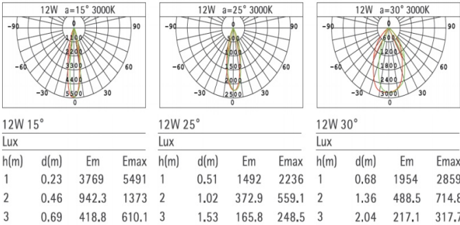
Figure 2- Adjustable CCT Light - Light Distribution
