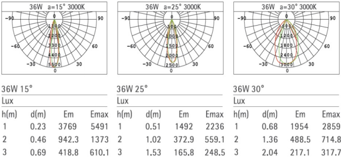
Figure 2- Adjustable CCT Light - Light Distribution
