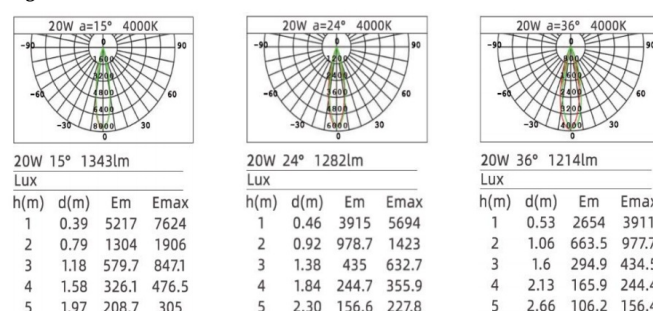
Figure 3- Fixed CCT Light - Light Distribution
