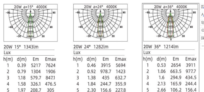
Figure 2- Adjustable CCT Light - Light Distribution
