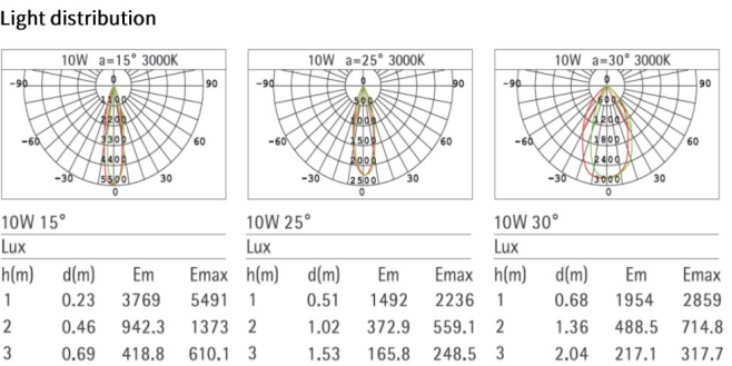
Figure 3- Fixed CCT Light - Light Distribution
