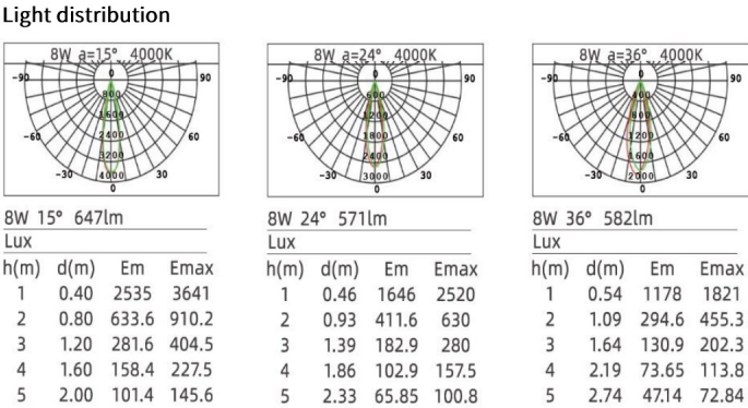
Figure 2 - Fixed CCT Light - Light Distribution
