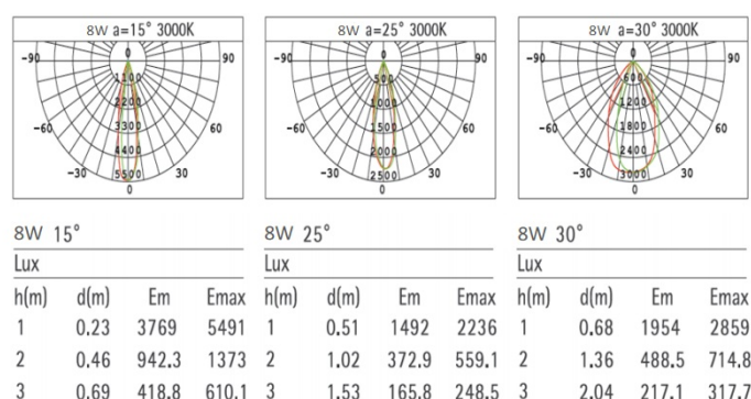
Figure 2- Adjustable CCT Light - Light Distribution
