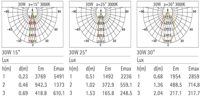
Figure 3- Fixed CCT Light - Light Distribution
