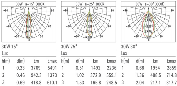
Figure 2- Adjustable CCT Light - Light Distribution
