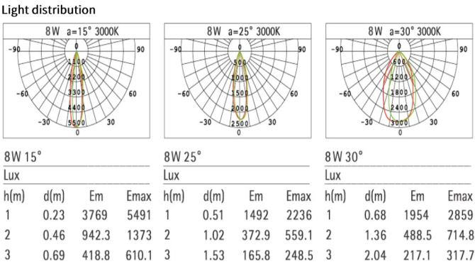
Figure 2 - Light Distribution
