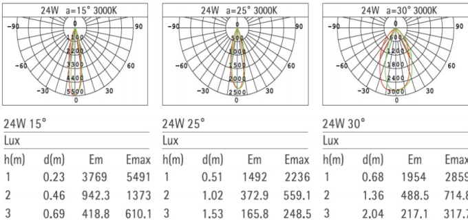
Figure 2- Fixed CCT Light - Light Distribution
