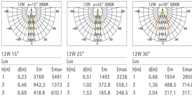
Figure 2- Fixed CCT Light - Light Distribution
