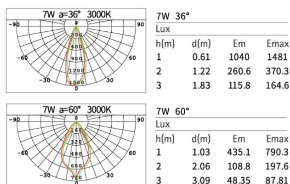
Figure 3- Fixed Color Temperature - Light Distribution
