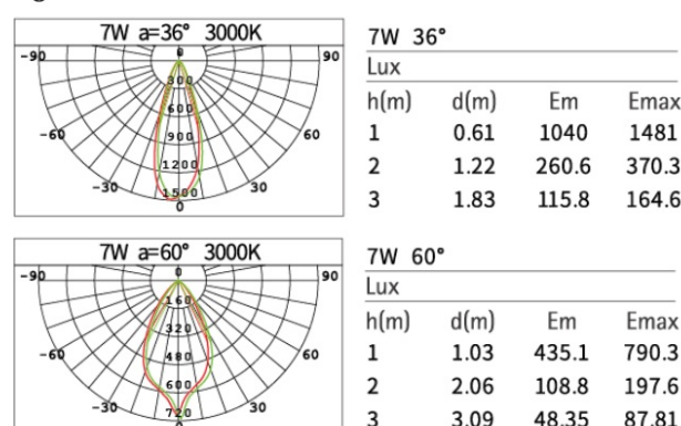
Figure 2- Adjustable Color Temperature - Light Distribution
