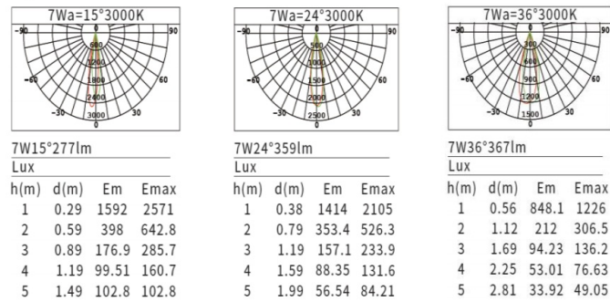
Figure 3- Fixed Color Temperature - Light Distribution
