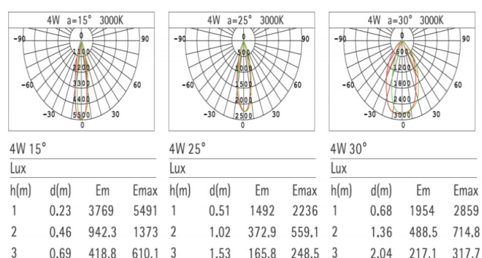
Figure 2- Fixed CCT Light - Light Distribution
