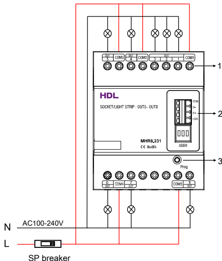
Figure 4. Wiring
