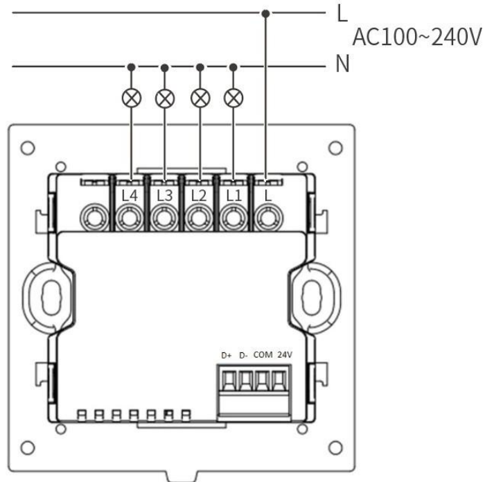
Panel power interface with 4CH relay
