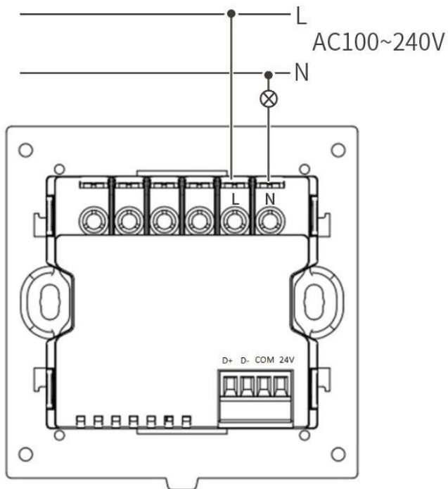
Panel power interface
