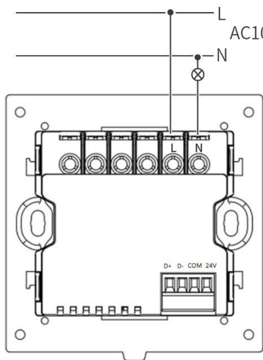
Panel power interface
